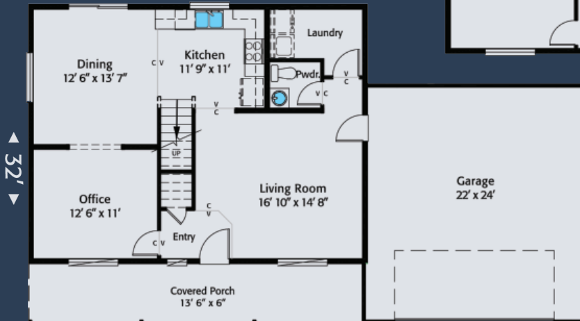
First Floor ▶ 56' ◀
