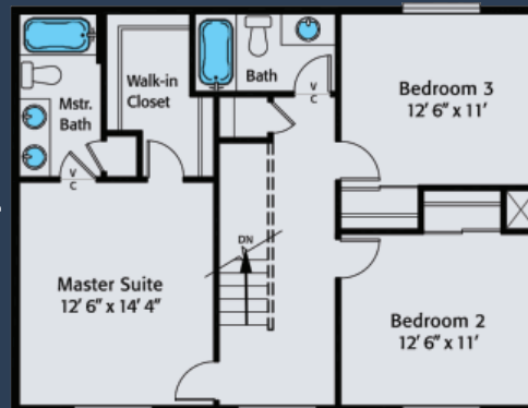
◀ 34' ▶ Second Floor
