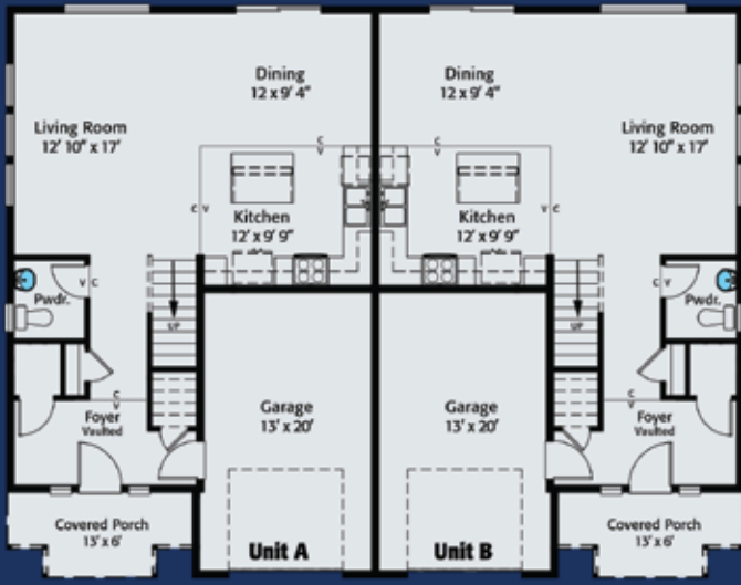
First Floor ◀ 51' 6 1/2" ▶
